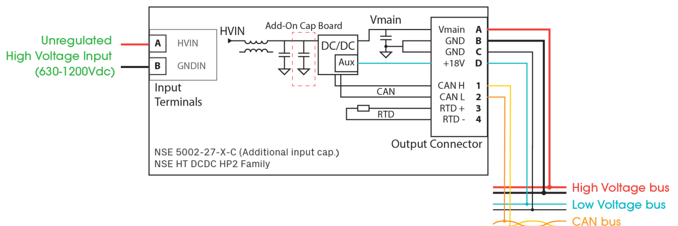
Figure 3 –Option -CX -Additional input capacitance
