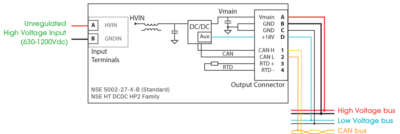
Figure 2 – Option - BX -Standard version (No telemetry)
