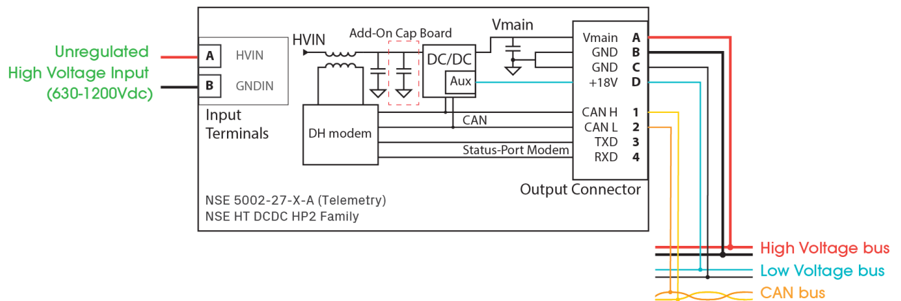
Figure 1 – Option-AX - Integrated telemetry
