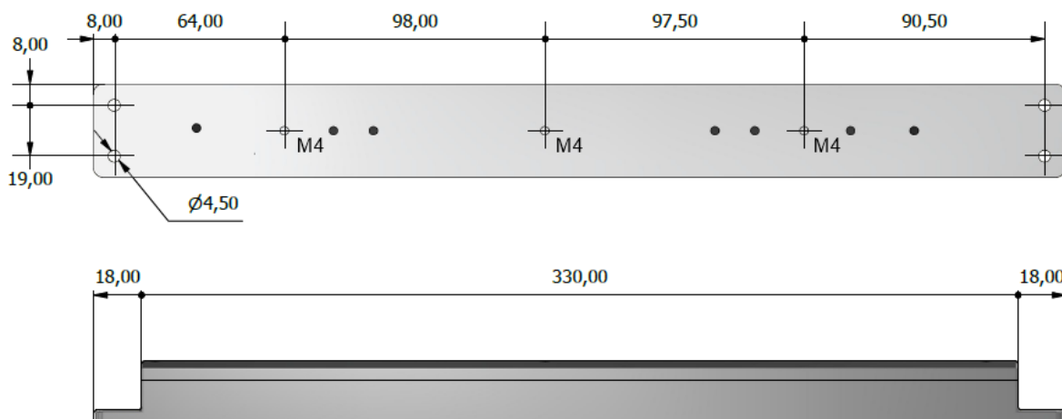
Figure 1 Mechanical dimensions
