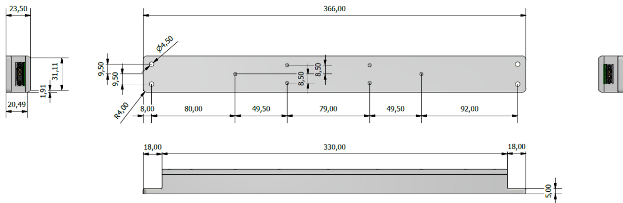
Figure 1 Mechanical dimensions
